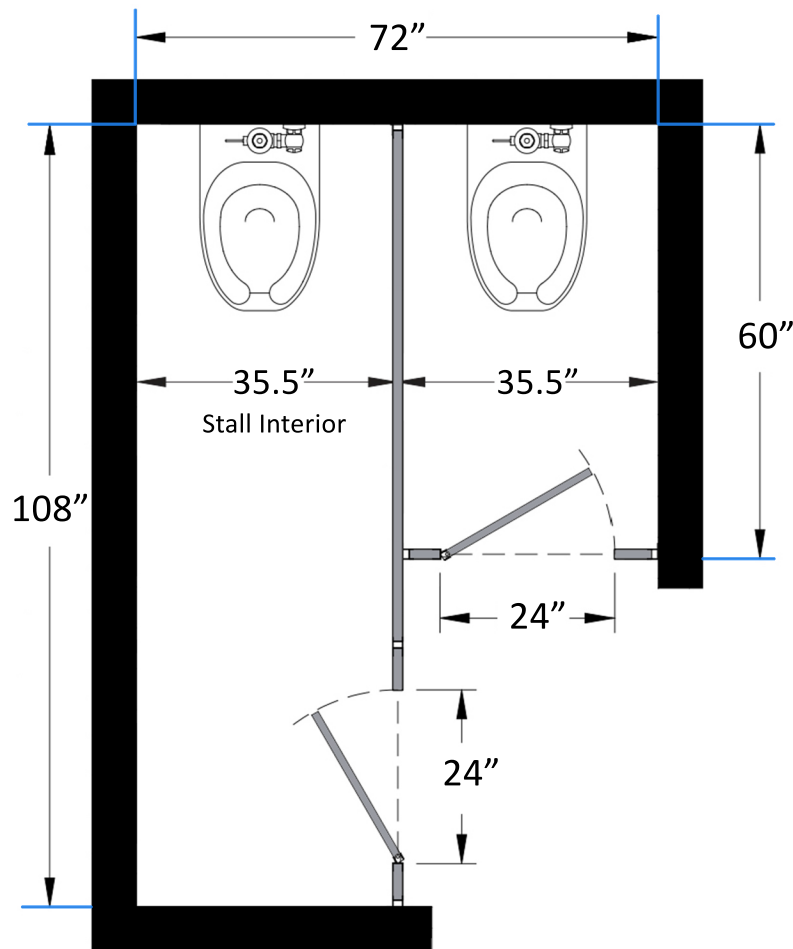
Bathroom Partitions - 2 Stall Alcove Left Hand SKU: AL2L Standard Dimensions
